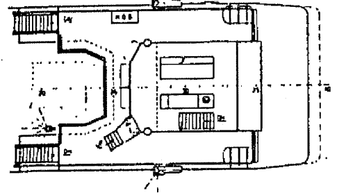
BOATDECK
