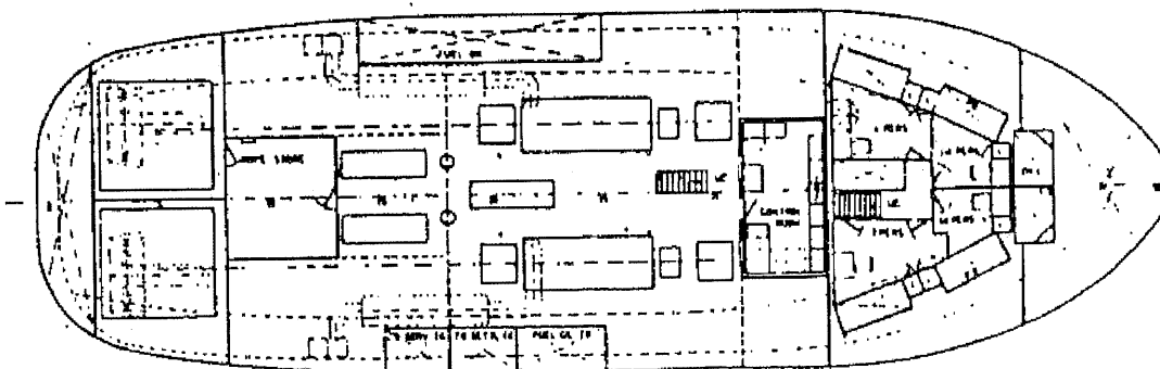
BELOW MAINDECK
